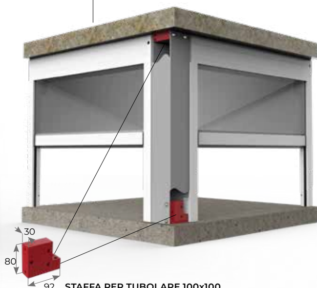
STAFFA PER TUBOLARE 100x100
